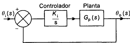
Figura 10.5 Control integral
