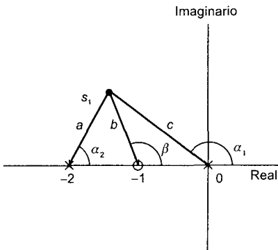
Figura 9.12 G_o(s) = K(s+1)/s(s+2)
