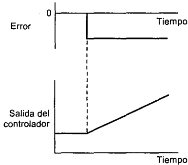
Figura 10.4 Control integral
