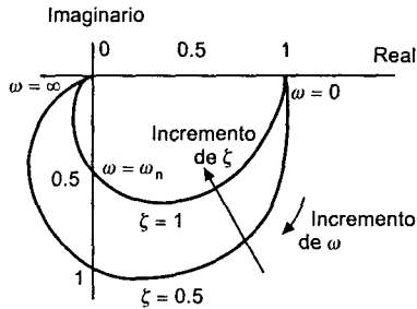
Figura 11.21 Trazado de Nyquist para G(s) = \omega_n^2 / (s^2 + 2\zeta\omega_n s + \omega_n^2)
