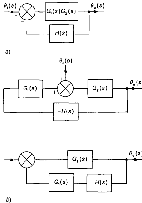
Figura 6.16 a) \theta_d(s) = 0 , b) \theta_i(s) = 0
