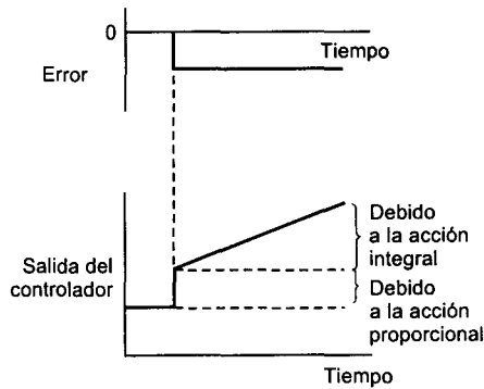
Figura 10.8 Control proporcional integral
